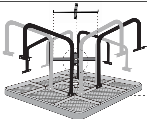
Step 1 Assembly of the Legs and table top
